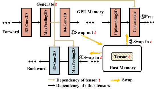
Fig. 2. A part of the architecture of U-Net. Tensor t is optimized for the host checkpoint.
